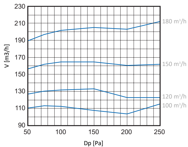
KVR-R 125 100-180 M3/H
