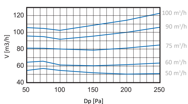
KVR-R 125 15-50 M3/H
