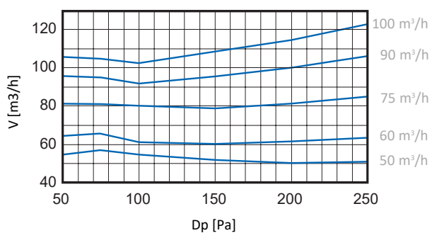
KVR-R 100 50-100 M3/H
