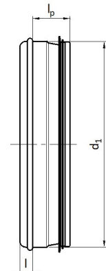
DDG 100 - 315
