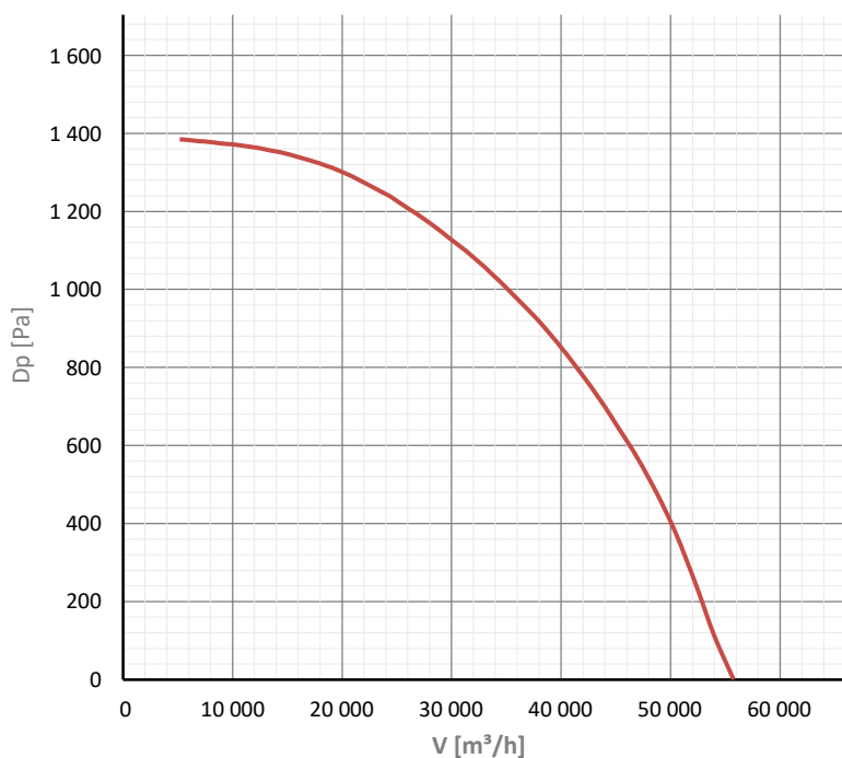
ROOF-HM 1006 T
