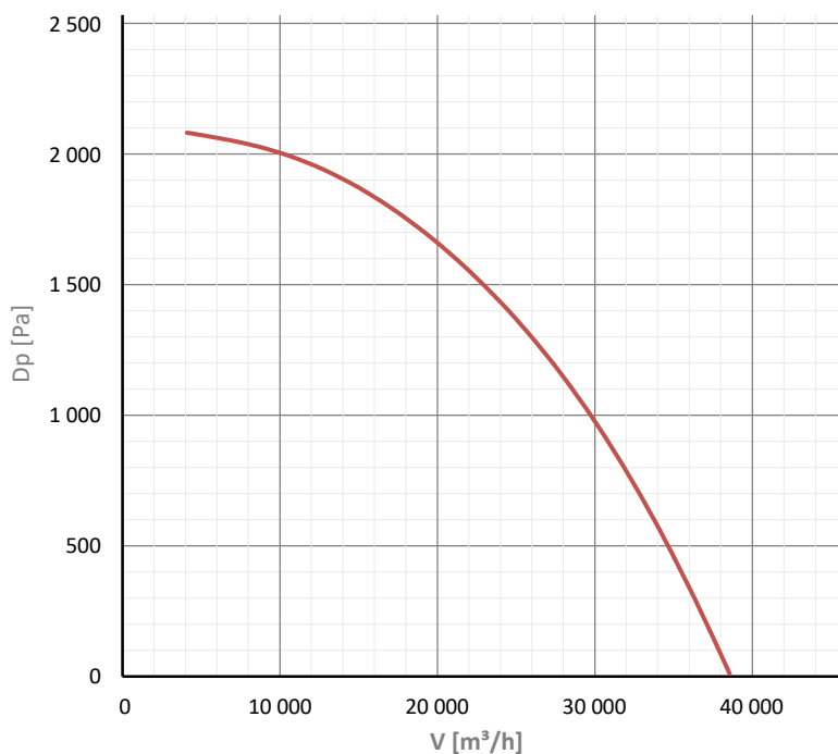
ROOF-HM 804 T
